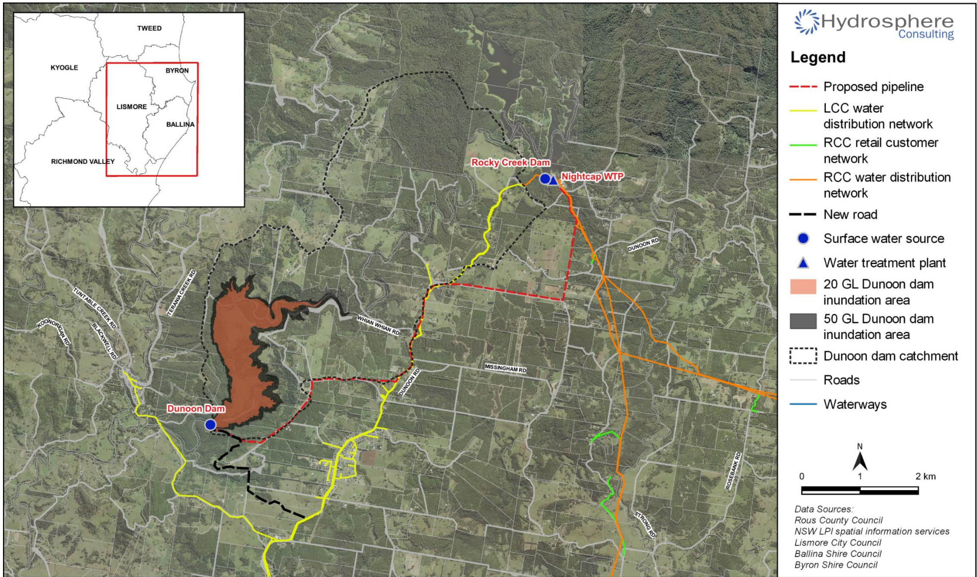
Figure 8: Dam location and inundation area for 20 GL and 50 GL storage options
